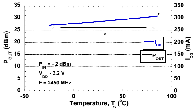
Output Power and Drain Current vs. Temperature at V_{DD} = +3.2\text{ V}
