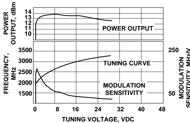
Figure 5. VTO-8200 Power Output, Frequency and Modulation Sensitivity vs. Tuning Voltage.
