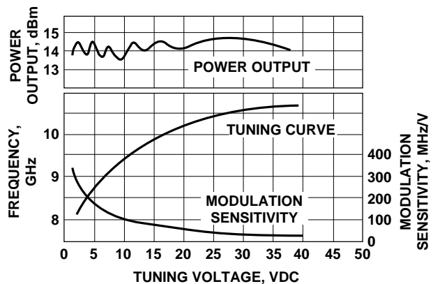
Figure 12. VTO-8850 Power Output, Frequency and Modulation Sensitivity vs. Tuning Voltage.
