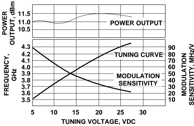
Figure 7. VTO-8360 Power Output, Frequency and Modulation Sensitivity vs. Tuning Voltage.
